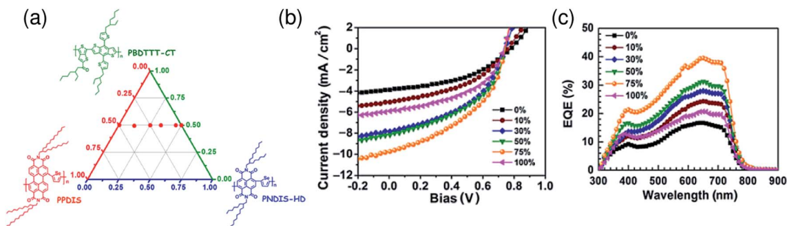
Fig. 27 (a) Composition of the ternary [PBDTTT-C-T] 1 [PPDIS] x [PNDIS-HD] 1-x blend illustrated on a ternary diagram. (b) J - V characteristics and (c) EQE spectra as functions of [PPDIS] x composition, where x is the PPDIS weight fraction in the binary acceptor components ( x = 0.10, 0.30, 0.50, 0.75 ). Reproduced with permission from (ref. 140). Copyright 2015, Materials Research Society.
