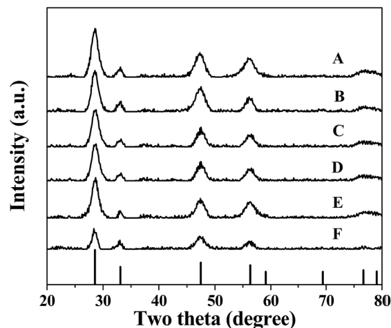
Fig. 5 XRD patterns of (A) Cu–CeO 2 –Pt; (B) Cu 0.66 Co 0.34 –CeO 2 –Pt; (C) Cu 0.50 Co 0.50 –CeO 2 –Pt; (D) Cu 0.34 Co 0.66 –CeO 2 –Pt; (E) Co–CeO 2 –Pt; (F) CeO 2 –Pt.
