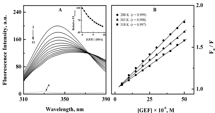
Fig. 2 (A) Fluorescence quenching spectra of 3 \text{ }\mu\text{M} HSA (spectrum 1) with increasing concentrations ( 5\text{--}50 \text{ }\mu\text{M} with 5 \text{ }\mu\text{M} intervals) of GEF (spectra 2–11), obtained in 60 \text{ mM} sodium phosphate buffer, \text{pH } 7.4 at 15 \text{ }^\circ\text{C} upon excitation at 295 \text{ nm} . The dotted line at the bottom (a) shows the fluorescence spectrum of GEF alone. Inset displays the decrease in the relative fluorescence intensity of HSA at 343 \text{ nm} ( F_{343 \text{ nm}} ) with increasing GEF/HSA molar ratios. (B) Stern–Volmer plots for the binding of GEF to HSA, obtained at three different temperatures, i.e., 288, 303 and 318 \text{ K} .
