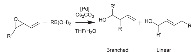
Scheme 3 Vinyl epoxide and boronic acid coupling.
