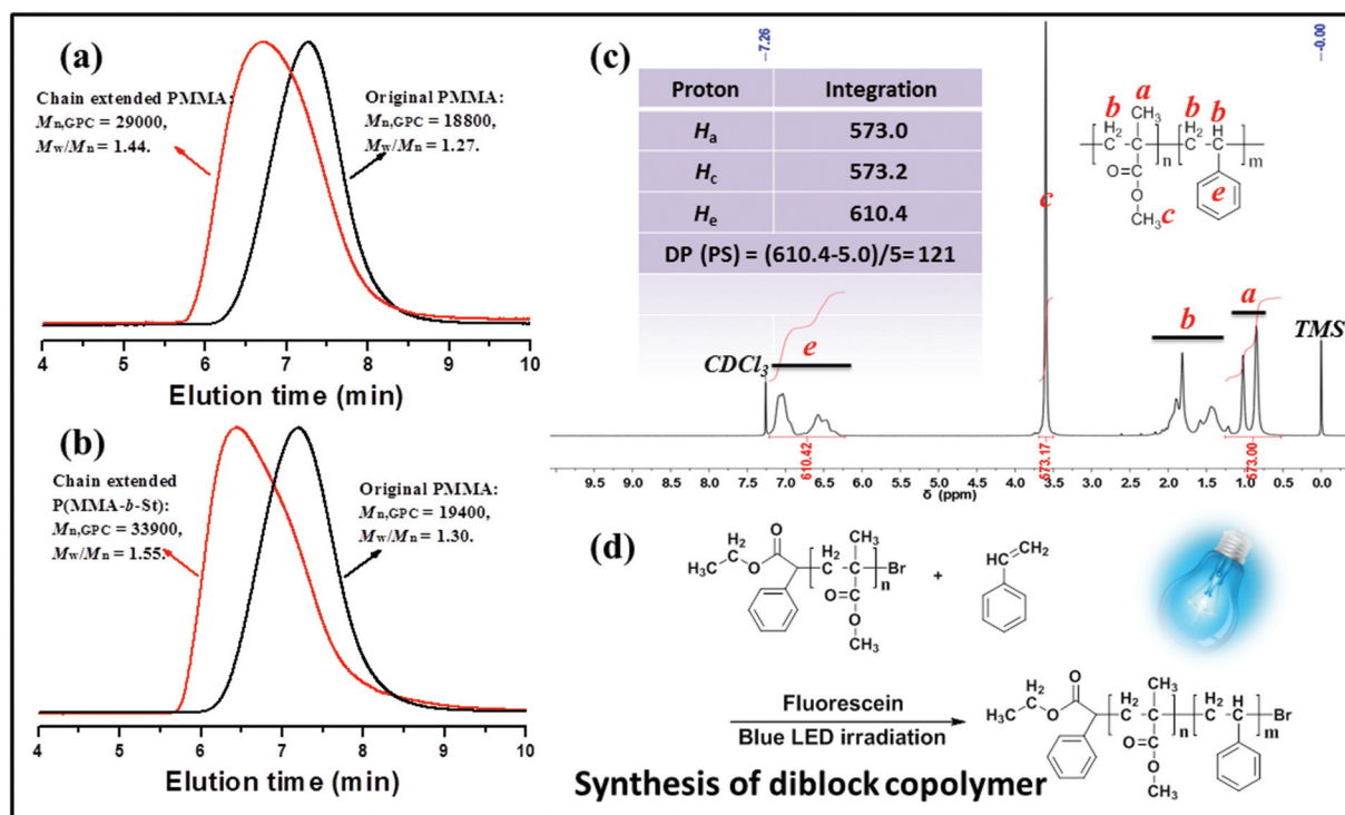
Fig. 7 (a) GPC traces of PMMA before and after chain extension using PMMA ( M_{n,GPC} = 18800 \text{ g mol}^{-1} , M_w/M_n = 1.27 ) prepared by metal-free PET-ATRP of MMA as the macroinitiator. (b) GPC traces of a poly(methyl methacrylate)- b -(styrene) diblock copolymer P(MMA- b -St) before and after chain extension using PMMA ( M_{n,GPC} = 19400 \text{ g mol}^{-1} , M_w/M_n = 1.30 ) prepared by metal-free PET-ATRP of MMA as the macroinitiator. (c) ^1H NMR spectrum of P(MMA- b -St) in CDCl_3 . (d) Synthesis of P(MMA- b -St) by the photoinduced metal-free PET-ATRP mechanism.
