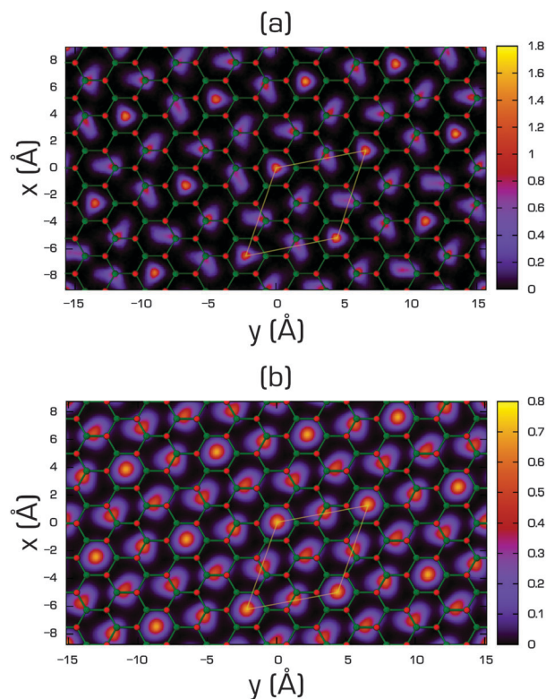
Fig. 14 Helium density (in Å -2 ) on the x – y plane of the 2/7 phase of 4 He on fluorographene (a) and on graphane (b) compared with the geometry of the substrate. Small red balls are centred on the position of fluorine/hydrogen atoms and the small green ones on the carbon atoms. Thin white lines enclose the unit cell of the commensurate 2/7 phase [reprinted with permission from ref. 305. Copyright 2012 by the American Physical Society].
