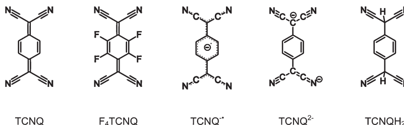
TCNQ structures
