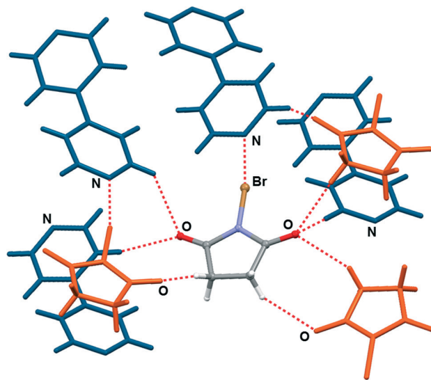
Fig. 3 Halogen and hydrogen bonding of nbs molecule with neighbouring molecules in the crystal structure of (nbs)(bpy) .
