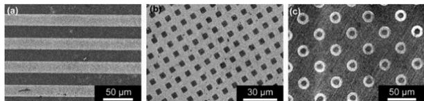
Fig. 7 SEM images of several Ag patterns fabricated by microcontact printing of (3-mercaptopropyl)triethoxysilane (MP TES) followed by selective electroless plating. (a) Lines with a width of 20 \mu\text{m} and 40 \mu\text{m} pitch, (b) a regular grid with 5 \mu\text{m} -wide lines and (c) rings with an internal diameter of 10 \mu\text{m} and an external diameter of 20 \mu\text{m} . Reprinted with permission from Mondin et al. 75 Copyright (2013) Elsevier.
