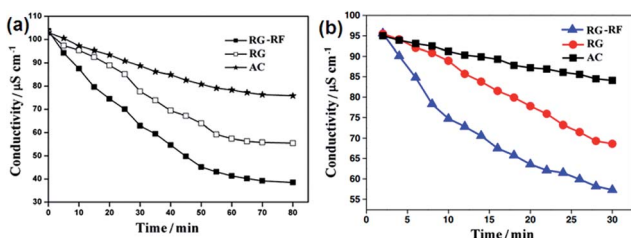
Fig. 25 Comparative results of RGO-RF, RGO and AC electrodes in terms of electrosorption performance in (a) 40 \text{ mg L}^{-1} \text{FeCl}_3 solution and (b) 40 \text{ mg L}^{-1} \text{NaCl} solution. (Reproduced with permission from ref. 129 and 130.)
