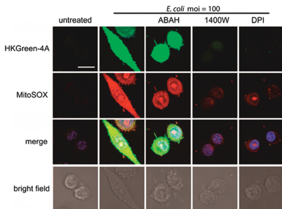
Fig. 70 Top: structure and reaction of HKGreen4 with \text{ONOO}^- . Bottom: images of RAW264.7 macrophages. Cells were co-treated with heat-killed E. coli moi = 100 and various enzyme inhibitors then stained with HKGreen4A , MitoSOX, and Hoechst 33342 before imaging. Aminobenzoic acid hydrazide (ABAH) is an inhibitor of myeloperoxidase that produces \text{ClO}^- ; 1400 W and DPI are inhibitors for iNOS and NOX, respectively. The merged images are overlays of all fluorescence channels. Scale = 10 \mu\text{m} . Image reproduced with permission. 287
