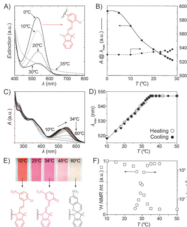
Fig. 9 Spiropyran as a probe for microenvironment polarity. (A) Thermally induced MC \rightarrow SP transition (0–30 °C) precedes precipitation of poly(NIPAM-SP) (35 °C). (B) Changes in maximum absorbance values and wavelength absorption maxima at temperatures below the volume phase transition. (C) Optical response of a poly(NIPAM-SP) polymer pre-irradiated with UV as it is gradually heated from T = 10^\circ\text{C} to T = 60^\circ\text{C} . (D) Temperature-dependent changes in wavelength absorption maxima of the same copolymer. (E) Colour changes accompanying a gradual zwitterion \rightarrow quinoid conversion (observed spectrophotometrically in (C)). (F) Precipitous drop of the integrated intensity of the NIPAM's CH proton resonances (left) coincides with the rapid increase of the hydrodynamic radius (right). [Adapted with permission from ref. 223 (Copyright 2004 American Chemical Society) (A and B) and ref. 224 (Copyright 2009 American Chemical Society) (C–F).]
