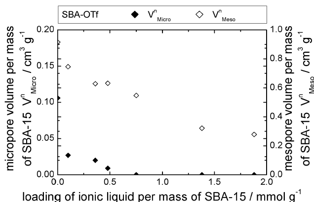
Fig. 12 Pore volume vs. loading of [C_6mim][OTf] on SBA-15.
