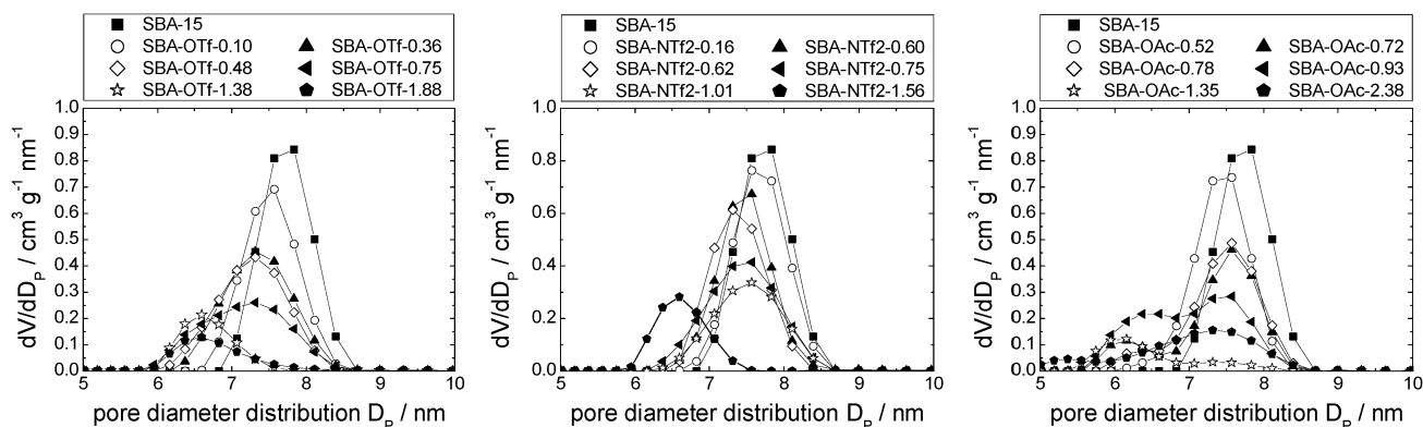
Fig. 13 Pore diameter distribution of SBA-15-based materials impregnated with incrementally increasing amounts of [C_6mim][OTf] (left), [C_6mim][NTf_2] (middle) and [C_6mim][OAc] (right).
