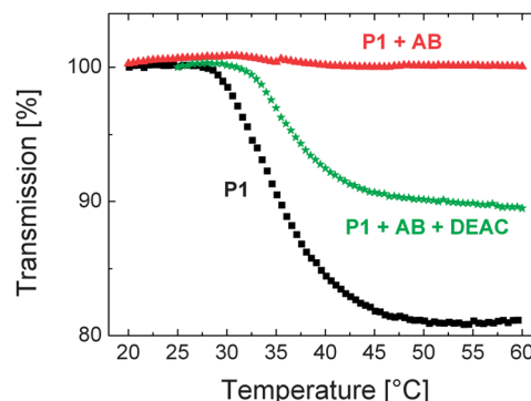
Fig. 7 Temperature–transmission profile of the aqueous solution of P1 ( 0.01 \text{ g L}^{-1} , black squares), containing 0.17 \mu\text{M} of antibody (red triangles), and containing both the antibody ( 0.17 \mu\text{M} ) and the DEAC-labelled monomer ( 4 \mu\text{M} ) (green stars). The profiles were recorded for the same solutions labelled a, b, and d of Fig. 6.
