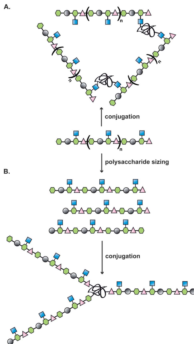
Fig. 1 Illustration of a classical approach to the design of a carbohydrate-based vaccine using polysaccharides extracted from biological sources; (A) direct conjugation to carrier protein; (B) polysaccharide sizing followed by end terminal conjugation of generated oligosaccharides.
