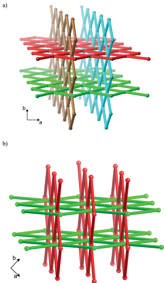
Fig. 7 Schematic representations of the interpenetration of “square-grid” sheets in a) \text{Cu}_2\text{imdc}_4\text{NaBF}_4 \cdot 7\text{H}_2\text{O} (5); b) \text{Zn}(4,4'\text{-bipy})_2\text{SiF}_6 \cdot 2\text{H}_2\text{O} . 8 Spheres represent metal centres whilst the bridging ligands are represented by the connections.
