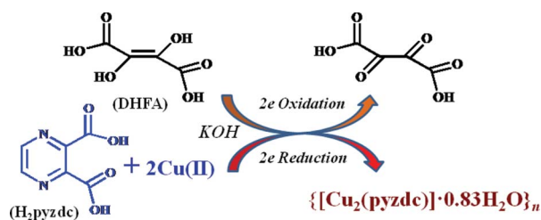
Scheme 1 Mechanism of the formation of \{[\text{Cu}_2(\text{pyxdc})]\cdot 0.83\text{H}_2\text{O}\}_n in presence of DHFA.
