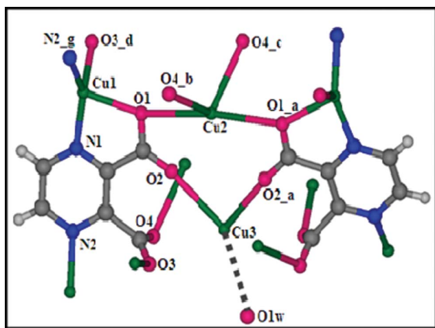
Fig. 1 View of the coordination environment around different Cu(I) centres connected by pyxdc in 1 . a = − x , y , −1/2 − z , b = − x , 1 − y , − z , c = x , 1 − y , −1/2 + z , d = x , 1 − y , 1/2 + z , g = 1/2 − x , 1/2 + y , 1/2 − z .
