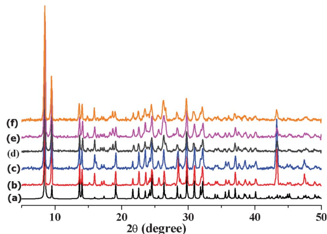
Fig. 3 PXRD pattern of compound 1 in different states. (a) simulated from single-crystal data; (b) as-synthesized \{[\text{Cu}_2(\text{pyxdc})]\cdot 0.83\text{H}_2\text{O}\}_n ; (c) dehydrated \{\text{Cu}_2(\text{pyxdc})\}_n ( 1' ); (d) rehydrated form of 1' ; (e) 1' exposed to the MeOH vapor and (f) 1' exposed to the MeCN vapor.
