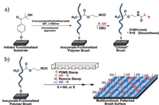
Fig. 1 (a) Schematic procedure for surface-initiated photopolymerization of 2-isocyanatoethyl methacrylate and subsequent X-isocyanate functionalization ( X = \text{thiol or amine} ). (b) Schematic procedure for patterning NCO-containing polymer brush surfaces with sequential X-isocyanate reactions.
