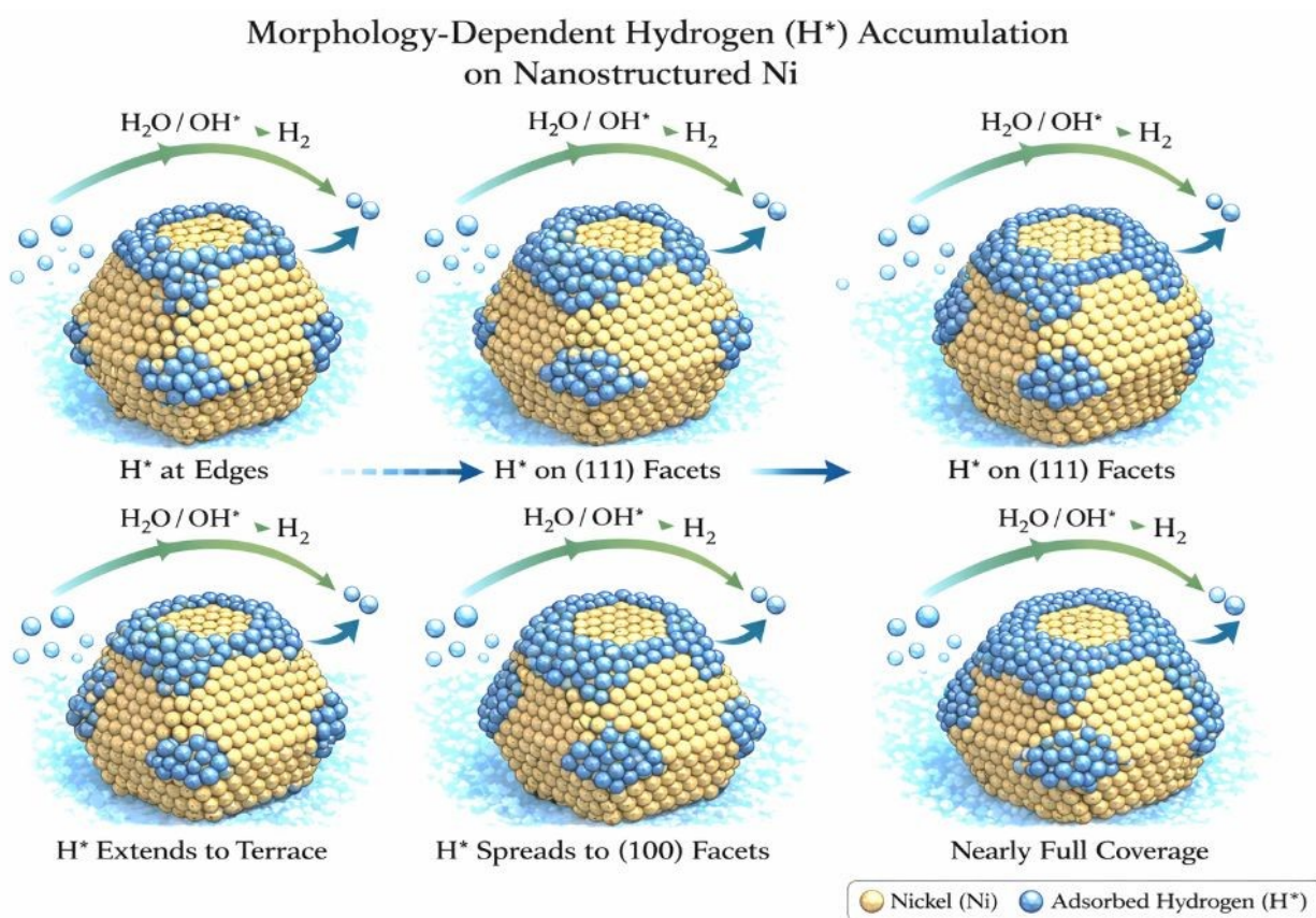
Figure 12. Morphology-dependent hydrogen utilization pathways on nanostructured Ni electrodes 99 .
