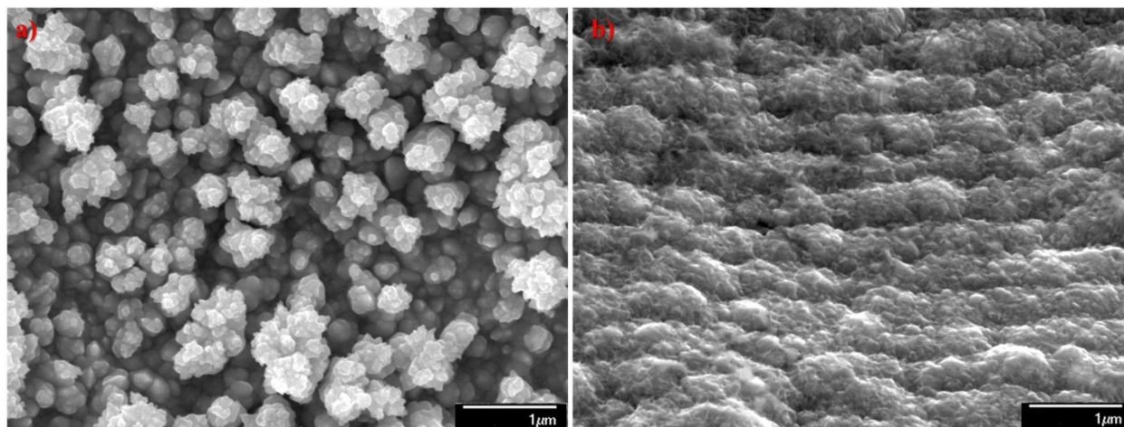
Figure 8. Ni electrodeposition on a) untreated Ni sheet, (b) laser nanostructured Ni sheet. Reprinted from Int. J. Hydrog. Energy Vol.47, Poimenidis, I. et al. Electrodeposited laser-nanostructured electrodes for increased hydrogen production, pp 9527-9536, Copyright (2022), with permission from Elsevier 40 .
