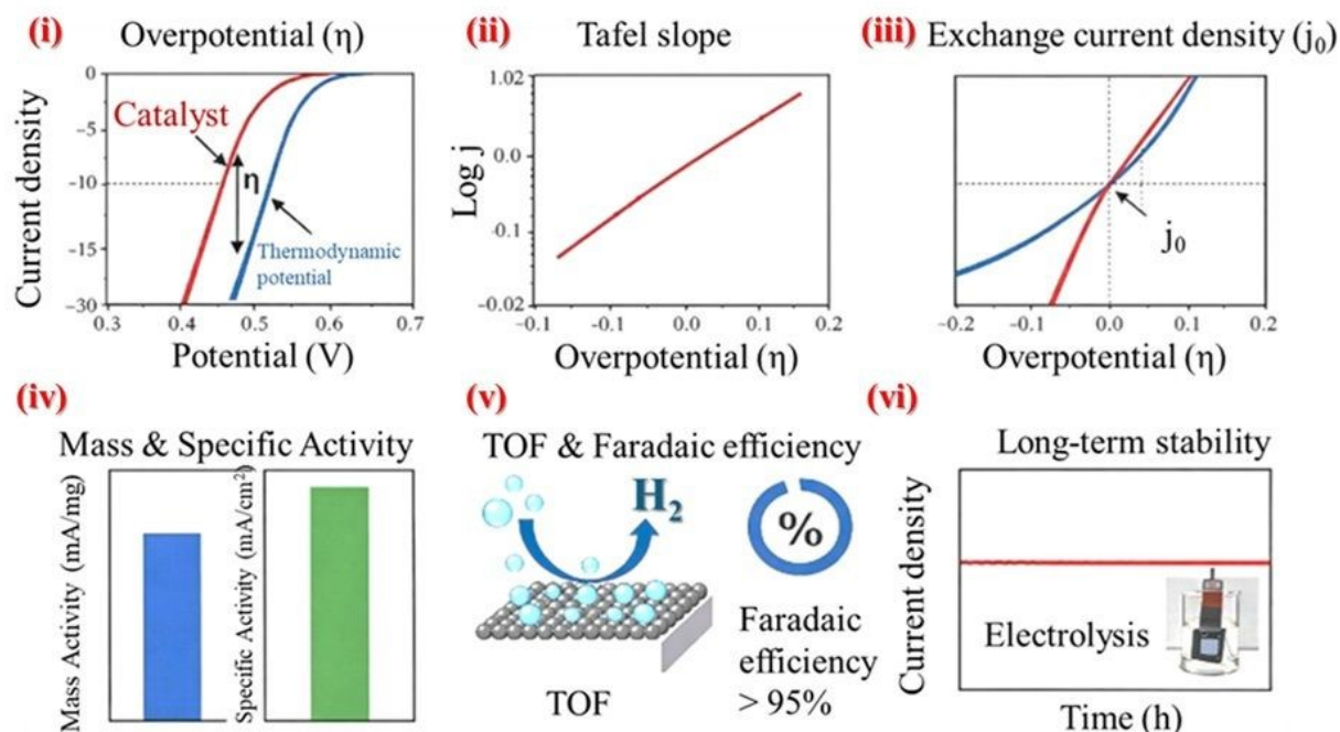
Figure 3. Schematic overview of the key parameters used to evaluate the catalytic performance of HER electrocatalysts.
