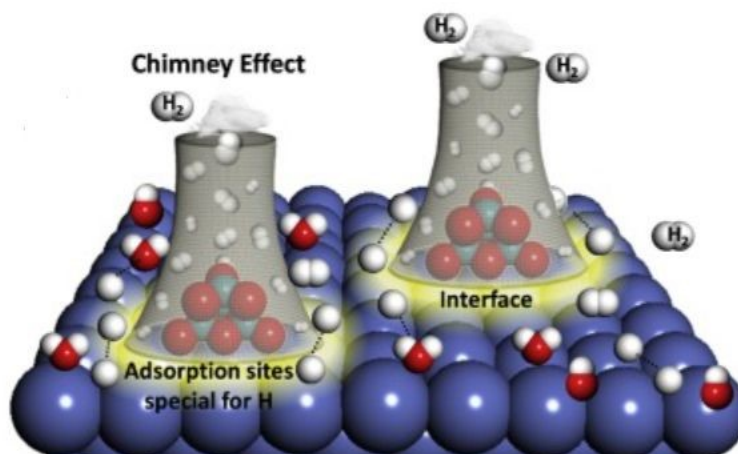
Figure 4. Schematic illustration of the “Chimney Effect” at the Ni/Oxide interface. Reprinted from Appl. Catal, B Environ. Vol.245, Peng, L. et al. Chimney effect of the interface in metal oxide/metal composite catalysts on the hydrogen evolution reaction, pp 122-129, Copyright (2023), with permission from Elsevier 49 .
