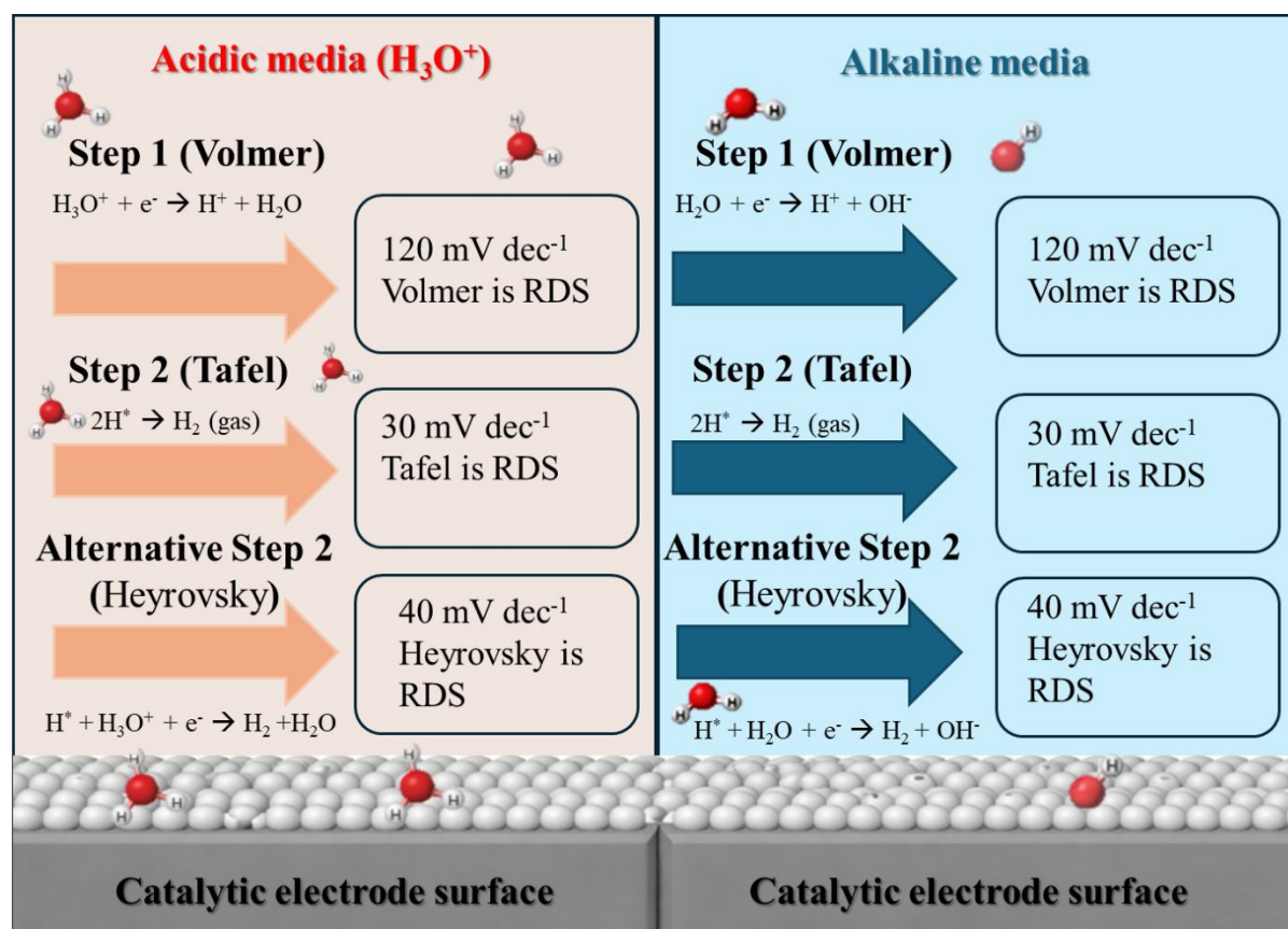
Figure 2. Comparison of HER Mechanisms and Theoretical Tafel Slopes
