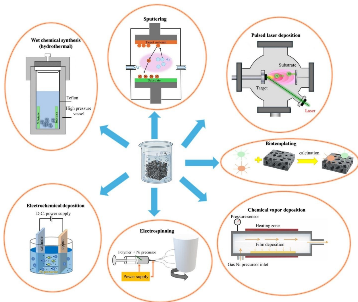
Figure 14. Schematic illustration of representative synthesis routes for monometallic Ni-based electrodes with tailored architectures for the hydrogen evolution reaction (HER).
