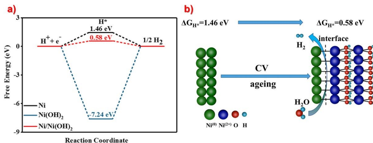
Figure 6. Calculated free energy for atomic hydrogen adsorption on Ni, Ni(OH) 2 , and Ni/Ni(OH) 2 and proposed mechanism for the enhanced HER on Ni/Ni(OH) 2 heterostructure. Reprinted from Int. J. Hydrog. Energy Vol.46, Lai, W. et al. In situ Raman spectroscopic study towards the growth and excellent HER catalysis of Ni/Ni(OH) 2 heterostructure, pp 26861-26872, Copyright (2021), with permission from Elsevier 56 .
