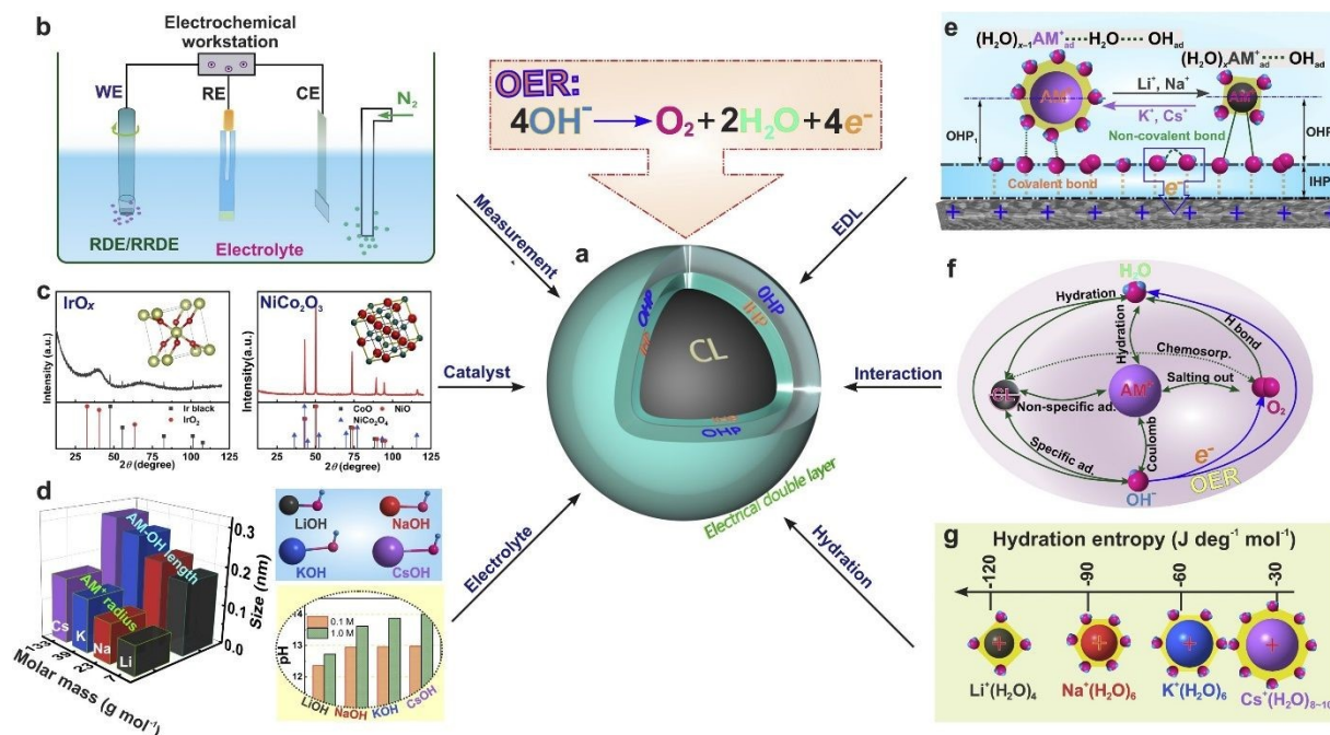
Figure 10. Schematic illustration of the electric double layer (EDL) in alkaline media, highlighting the distribution of solvated cations (AM + ), hydroxide species, and interfacial water molecules. The interaction between hydrated cations and adsorbed hydroxyl species (OH * ) at the outer Helmholtz plane influences the local electric field and hydrogen-bond network, thereby modulating water dissociation and HER kinetics. Applied Catalysis B: Environmental , Julie Anne D. del Rosario, Guangfu Li, Marc Francis M. Labata, Joey D. Ocon, Po-Ya Abel Chuang, Unravelling the roles of alkali-metal cations for the enhanced oxygen evolution reaction in alkaline media, Volume 288, 119981, Copyright (2021), with permission from Elsevier 92
