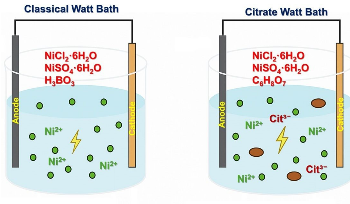
Figure 15. Electrodeposition of classical Ni Watt bath and modified citrate Watt bath.
