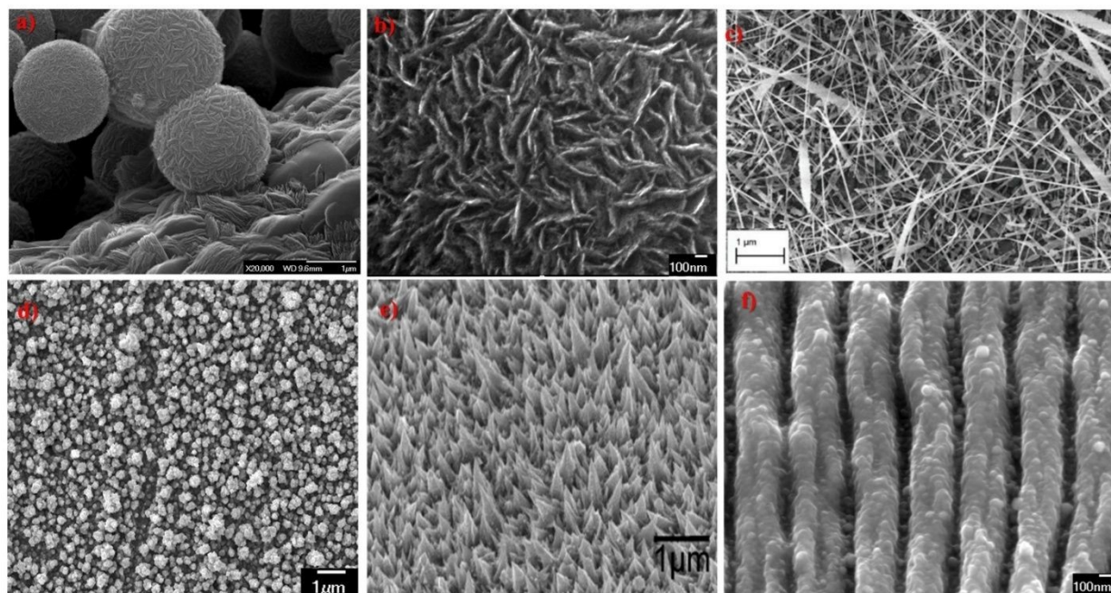
Figure 11. Various Ni-based morphologies: Nanoworms (a, b) 22 , nanowires (c) 95 , nanoparticles (d), nanocones (e) 94 , protrusions (f) 16 . Reprinted from Mater. Chem. Phys. Poimenidis, I. et al. One-step solvothermal growth of NiO nanoparticles on nickel foam as a highly efficient electrocatalyst for hydrogen evolution reaction. Vol. 305, pp. 128007, Copyright (2023), with permission from Elsevier (a, b). Reprinted from Procedia Eng. , Kaur, N., Comini, E., Poli, N., Zappa, D. & Sberveglieri, G., Nickel Oxide Nanowires Growth by VLS Technique for Gas Sensing Application. Vol. 120, pp. 760-763, Copyright (2015), with permission from Elsevier (c). Reprinted from J. Power Sources . Du, Z., Zhang, S., Xing, Y. & Wu, X., Nanocone-arrays supported tin-based anode materials for lithium-ion battery. Vol. 196, pp. 9780-9785, Copyright (2011), with permission from Elsevier (e). Reprinted from Int. J. Hydrog. Energy , Poimenidis, I. A. et al. , Enhanced hydrogen production through alkaline electrolysis using laser-nanostructured nickel electrodes. Vol. 46, pp. 37162-37173, Copyright (2021), with permission from Elsevier (f).
