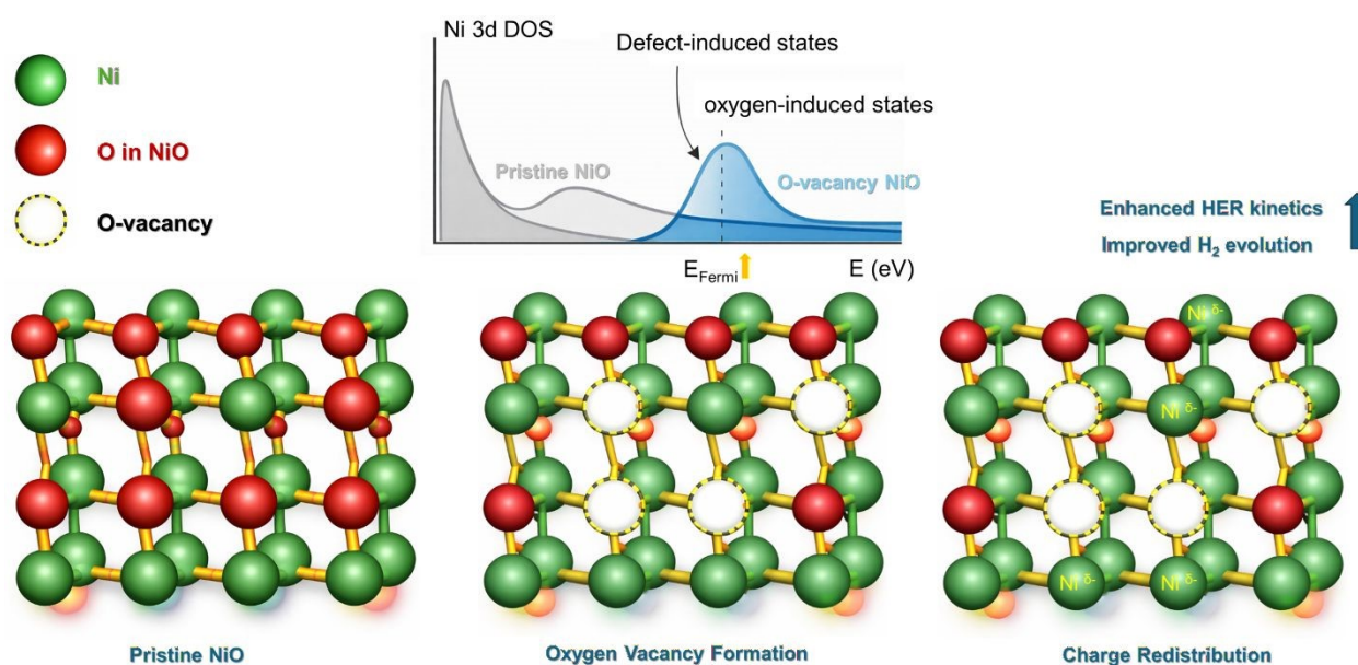
Figure 13. Schematic representation of the Ni 3d density of states (DOS) for pristine NiO and oxygen-deficient NiO with oxygen vacancies and charge redistribution. Adapted conceptually from 101,103
