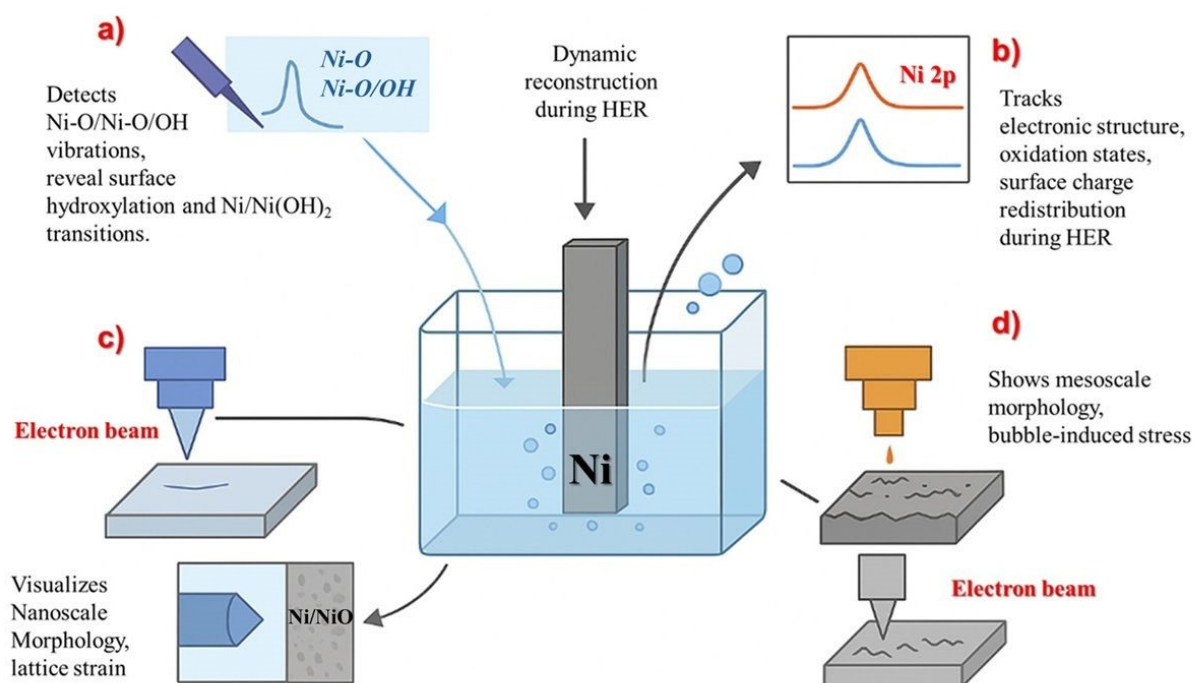
Figure 5. Operando techniques applied for characterization of Ni-based electrodes: Raman (a), XPS (b), TEM (c), SEM (d).
