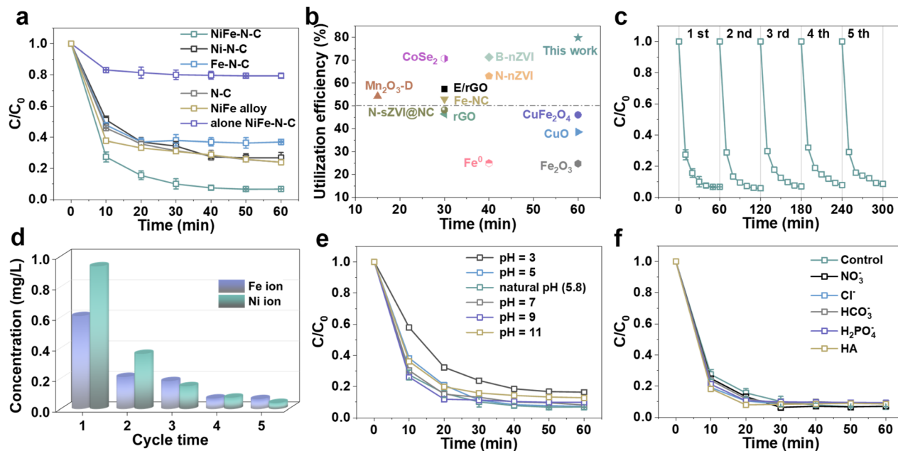
Fig. 3 (a) TC degradation in PMS activation with different catalysts; (b) comparison of \text{UE}_{\text{PMS}} in different catalytic systems; (c) successive cyclic runs of TC degradation in the NiFe-N-C/PMS system; (d) leaching concentrations of Fe and Ni ions during successive cyclic runs; (e) effect of initial pH on TC degradation; and (f) effect of the co-existence of inorganic anions and humic acid on TC degradation in the NiFe-N-C/PMS system. Reaction conditions: m_{\text{catalyst}} = 20 \text{ mg} , [\text{TC}]_0 = 10 \text{ mg L}^{-1} , [\text{oxidant}] = 1 \text{ mM} , natural pH and T = 298 \text{ K} .
