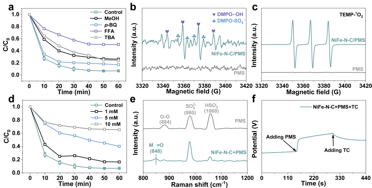
Fig. 4 (a) TC degradation with different kinds of scavengers; EPR spectra of (b) DMPO-·OH and DMPO-SO 4 · - , and (c) TEMP- 1 O 2 ; (d) quenching experiments of the NiFe-N-C/PMS systems by using DMSO; (e) Raman spectra of PMS and NiFe-N-C/PMS systems; (f) open-circuit potential tests.
