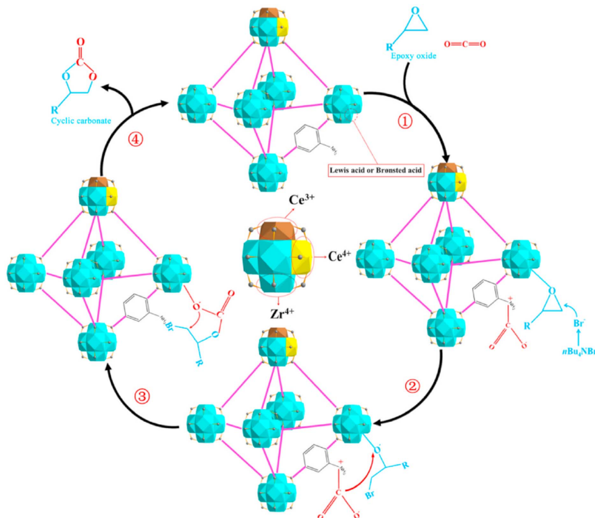
Fig. 16 Proposed mechanism for the cycloaddition of \text{CO}_2 and epoxides by a defective bimetallic \text{UiO}-66-\text{NH}_2(\text{Zr}/\text{Ce}) catalyst. (1) Through the catalyst, epoxy oxide is integrated with Lewis or Brønsted acid sites and is activated. Due to the presence of the -\text{NH}_2 group on the MOF, \text{CO}_2 is adsorbed and polarized; (2) the nucleophilic \text{Br}^- ion attacks the \beta carbon atom of epoxy to form the oxygen anion intermediate; (3) the intermediate interacts with \text{CO}_2 to create halogenated carbonate; (4) through internal cyclization, halogenated carbonate is converted into cyclic carbonate, while the catalyst is regenerated. Reproduced with permission from ref. 293, copyright 2021 Elsevier.
