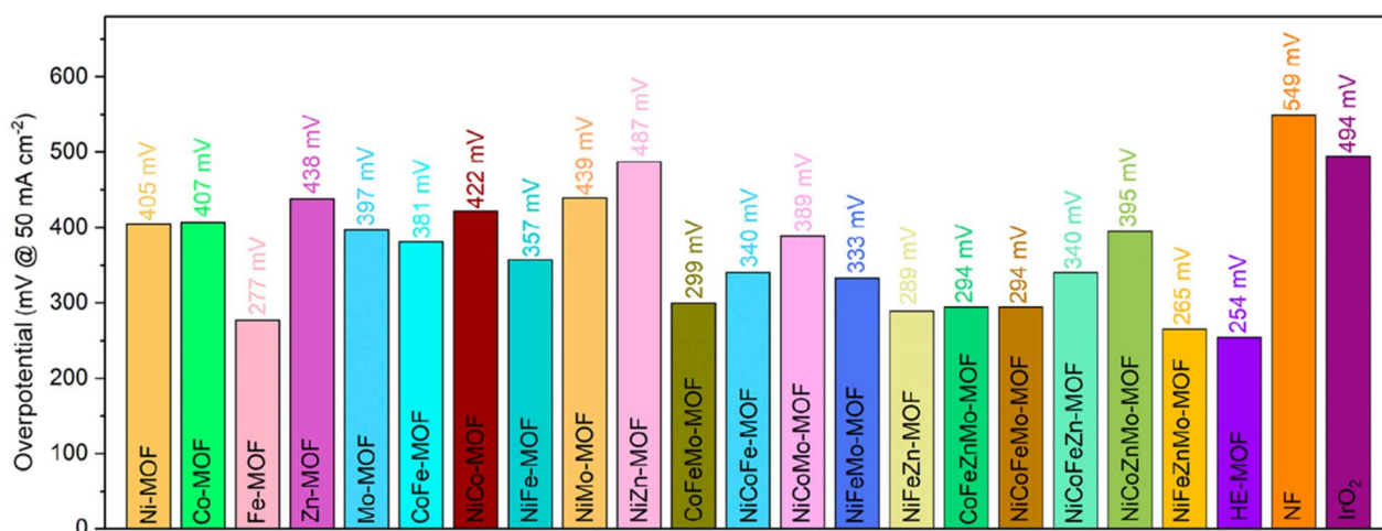
Fig. 12 Comparison of the overpotential of HE-MOF with other mono-, bi-, tri-, and tetra-metallic MOFs, bare NF, and commercial \text{IrO}_2 solids. Reproduced with permission from ref. 171, copyright 2022 American Chemical Society.
