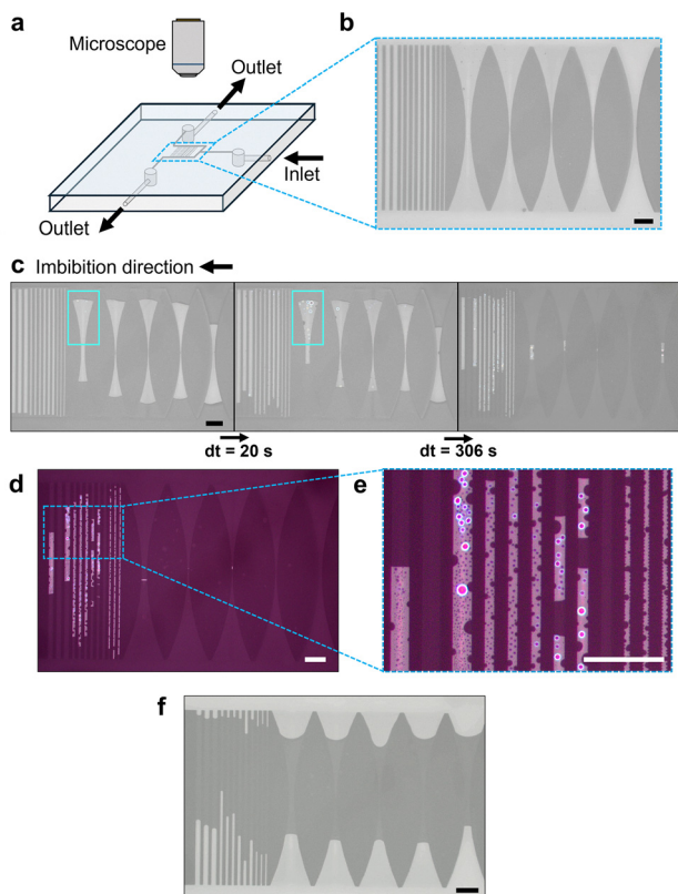
Fig. 4 (a) Schematic of experimental setup for imbibition and drainage experiments in a PDMS-glass chip. Brightfield microscope images of the microfluidic chip (b) before imbibition, (c) during imbibition, and (d and e) at steady state \sim 30 min after commencing imbibition show air bubbles trapped by liquid in the central channels. The cyan rectangles in (c) point out water condensation inside the air bubbles. (f) Brightfield microscope image of a drainage experiment, in which liquid was trapped inside the central channels. All scale bars are 50 \mu\text{m} .
