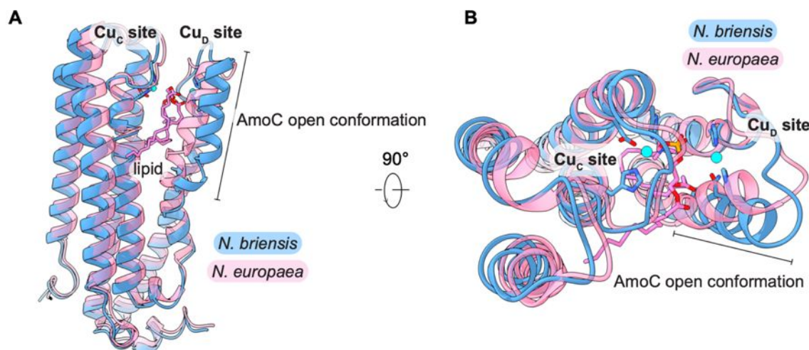
Figure 4. Superposition of the AmoC subunits from the N. europaea (pink) and N. briensis (blue) AMO structures in native membranes. Ligands to the Cu C and Cu D sites in N. briensis AMO are shown as sticks and copper ions are shown as cyan spheres. Only the Cu C site is occupied in the N. europaea AMO structure.
