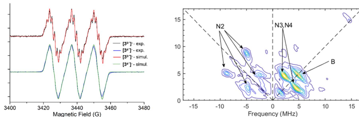
Fig. 4 EPR spectra of [3^a]^- and [3^b]^- in solution at room temperature, together with their corresponding numerical simulations (left) and HYSORE spectrum of [3^b]^- recorded at T = 70 K (right).
