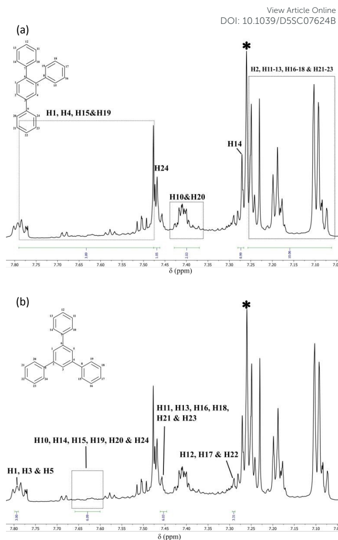
Figure 6. The spectra in (a) and (b) are duplicated here, to allow presentation of the assignments for both isomers more clearly. (a) ^1\text{H} NMR (25 °C, d -chloroform, 700 MHz) spectrum of a mixture of 1,2,4- and 1,3,5-triphenylbenzene prepared using a 0.5 mol% precatalyst loading of 1f and [ \text{Ph}_3\text{C} ][ \text{B}(\text{C}_6\text{F}_5)_4 ] (cation 2f ) at room temperature, with the resonances for the 1,2,4-isomer highlighted. (b) The same spectrum with the resonances for 1,3,5-triphenylbenzene highlighted. * d -chloroform.
