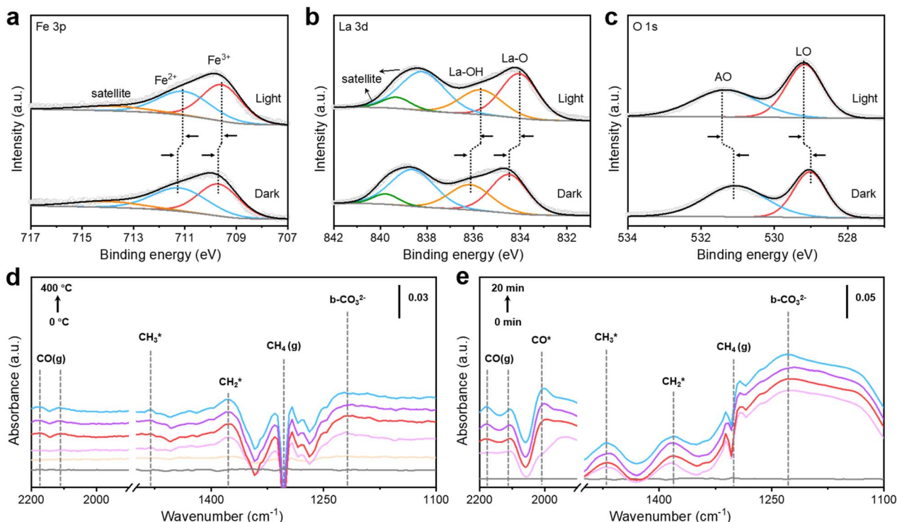
Fig. 4 ISI-XPS spectra of (a) Fe 3p, (b) La 3d and (c) O 1s of Ru/LaFeO 3 . (d and e) In situ DRIFTS spectra of Ru/LaFeO 3 catalysts in CO 2 /CH 4 -saturated atmosphere under (d) external heating and (e) light irradiation.
