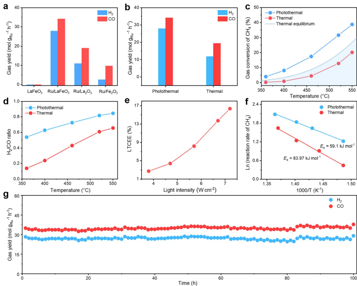
Fig. 2 (a) DRM performances of different catalysts under light-driven conditions (catalyst: 80 mg; light intensity: 6.7 W cm -2 ; feedstocks: CO 2 /CH 4 /He = 47/47/6, GHSV = 22.5 L g -1 h -1 ). (b) DRM activities of Ru/LaFeO 3 under photothermal and thermal conditions. (c) CH 4 conversion under photothermal and thermal conditions at different temperatures. (d) H 2 /CO ratios of DRM at different temperatures powered by pure light irradiation and external heating. (e) LTCEEs of Ru/LaFeO 3 under different incident intensities. (f) Arrhenius plots of CH 4 in photothermocatalysis and thermocatalysis by Ru/LaFeO 3 . (g) Stability test of Ru/LaFeO 3 in light-driven DRM.
