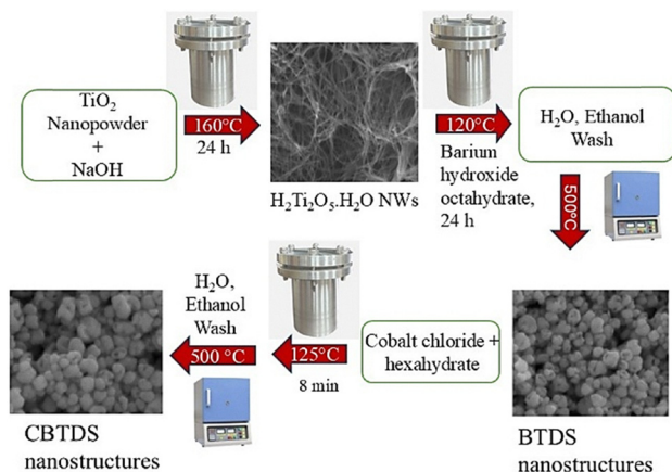
Scheme 1 Schematic of the steps involved in forming \text{H}_2\text{Ti}_2\text{O}_5\cdot\text{H}_2\text{O} nanowires and \text{BaTiO}_3 and \text{CoBaTiO}_3 doughnut nanostructures.
