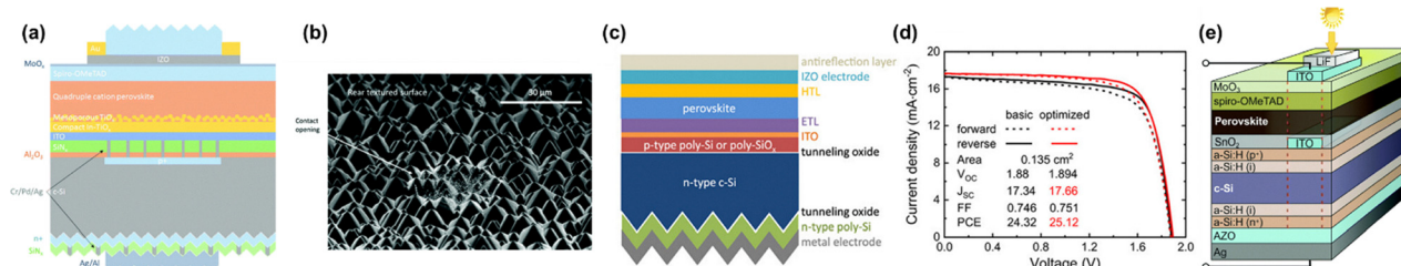
Fig. 9 (a) Structure of perovskite/PERC tandem solar cell with an intermediate contact of a Cr/Pd/Ag metal stack, and (b) SEM image of textured Si surface with local openings using the metal stack. Reproduced with permission. 53 Copyright 2017, The Royal Society of Chemistry. (c) Structure of a perovskite/TOPCon tandem solar cell incorporating a poly-SiO x layer, and (d) J - V characteristics comparing basic (using poly-Si) and optimized (using poly-SiO x ) configurations of the perovskite/TOPCon tandem solar cell. Reproduced with permission. 56 Copyright 2024, John Wiley and Sons. (e) Structure of perovskite/SHJ tandem solar cell with SnO 2 layer deposited using ALD. Reproduced with permission. 41 Copyright 2016, The Royal Society of Chemistry.
