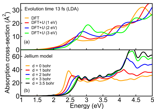
Fig. 5 (a) Variation in the TDDFT+ U absorption spectra of Au 309 as a function of the U parameter (0 to 3 eV), with the LDA (PZ81) 25 to approximate the XC functional (time evolution of 13 fs) and (b) variation in the absorption spectra calculated using the jellium model, with a reduced screening layer of different thicknesses (0 to 3.5 Bohr), as indicated in the legend ( \hbar\delta = 60 meV).
