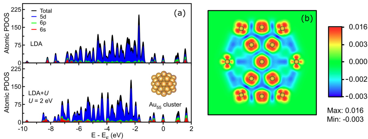
Fig. 4 (a) PDOS for the Au 55 cluster with and without an effective Hubbard- U correction of 2 eV. (b) Ground state total (5d + 6s) charge-density difference between DFT+ U (2 eV) and DFT for Au 55 , represented using a colour-coded slab passing through the central atom, confirming increased localization of the d electrons around atoms.
