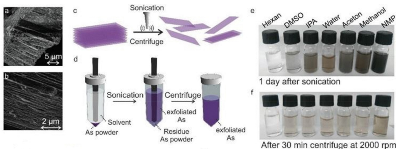
Fig. 21 Solvent exfoliation of arsenic via tip ultrasonication: (a) and (b) SEM images showcase the layered structure of bulk arsenic crystals. (c) The exfoliation process involves tip ultrasonication and subsequent centrifugation to isolate thin layers. (d) A schematic illustrating the tip ultrasonication setup designed to minimize exposure to ambient air, preserving material quality. (e) A photograph shows arsenene dispersions in various solvents one day post-ultrasonication, and (f) the dispersions after centrifugation at 2000 rpm, reproduced from ref. 141 with permission from John Wiley and Sons, copyright 2018.
