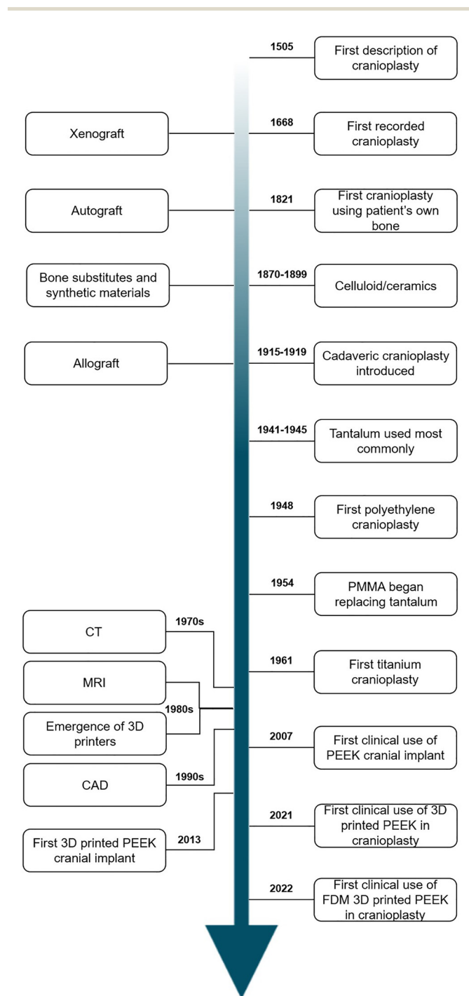
Fig. 3 Cranioplasty timeline.
