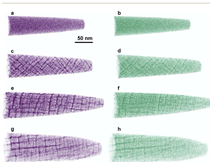
Fig. 8 AP composition profiles for Zr (purple) and Hf (green) from modified Senkov alloy ZrNbTaWf: (a) and (b) as-cast, and after annealing at 1800 °C for (c) and (d) 6 hours, (e) and (f) 1 day, and (g) and (h) 4 days (after Maiti and Steurer 43 ). Reproduced with permission from Elsevier from ref. 43.
