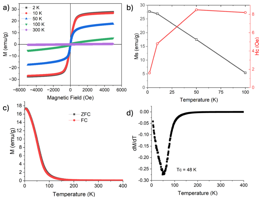
Fig. 6 Magnetic behaviour of the solution-annealed (SA) condition. (a) Isothermal magnetization ( M-H ) loops measured at multiple temperatures, showing ferromagnetic behaviour at low temperature and a paramagnetic behaviour at room temperature. (b) Temperature dependence of saturation magnetization ( M_s , left axis, black squares) and coercivity ( H_c , right axis, red circles). (c) Zero-field-cooled (ZFC) and field-cooled (FC) magnetization curves measured in a 1000 Oe applied field, revealing a single magnetic transition. (d) Derivative of magnetization ( dM/dT ) used to determine the Curie temperature, T_c \approx 48 K.
