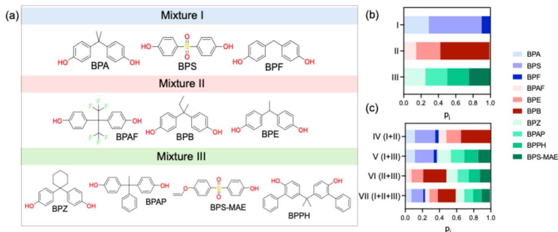
Fig. 1 (a) Schematic illustration of the three base mixtures I, II, III with chemical structures of the 10 mixture components (Table S3). (b) Representation of the mixture design and as stacked bar plots for mixture I with BPA, BPS and BPF coloured in blue, mixture II with BPAF, BPE, and BPB coloured in red, mixture III with BPZ, BPAP, BPPH and BPS-MAE in green. (c) The other mixtures I + II, I + III, II + III are combinations of the first three. Mixture I + II + III is a 10-component mixture. Data from Tables 1 and S3.
