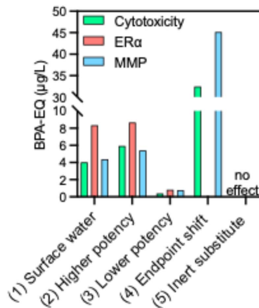
Fig. 5 Comparing the BPA-EQ(bioassay) of the endpoints median cytotoxicity (green), ER\alpha (red), mitochondrial membrane inhibition potential (MMP; blue) for five scenarios: (1) “surface water”, (2) “high-potency”, (3) “low-potency”, (4) “endpoint shift” and (5) “inert behavior” (data in Table S13).
