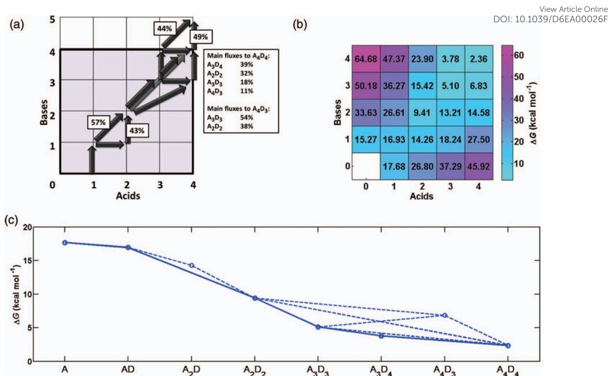
Figure 8. Main clustering pathways and Gibbs free energies of formation of the clusters in the electrically neutral sulfuric acid-DMA system at T = 5\text{ }^{\circ}\text{C} , [\text{SA}] = 10^6\text{ cm}^{-3} and [\text{DMA}] = 1\text{ ppt} , Panel (a): Major routes leading out of the simulated system. For figure clarity, the arrows that fall on top of each other are colored with different shades. Panel (b): Formation free energies of a cluster in the system. Panel (c): formation free energy of the growing cluster as a function of growth step. Solid and dashed lines: correspond to the major and minor fluxes, respectively. Adapted from Olenius et al., 2013 76 . Reproduced from ref. 76 with permission from the AIP Publishing, copyright 2013.
