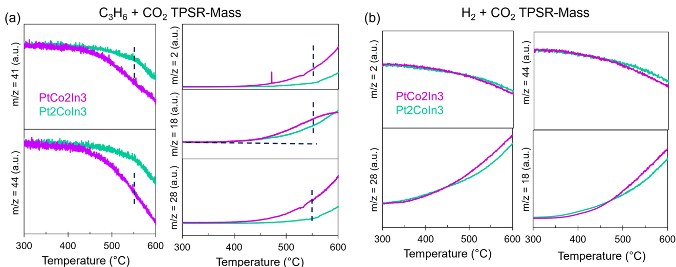
Fig. 4 Temperature-programmed surface reactions (TPSRs) on the PtCo2In3/CeO 2 and Pt2CoIn3/CeO 2 catalysts. (a) C_3H_6 + CO_2 TPSR-mass experiments (b) and H_2 + CO_2 TPSR-mass experiments. The reactants and products were collected with the mass intensity of m/z = 2 ( H_2 ), m/z = 18 ( H_2O ), m/z = 28 (CO), m/z = 41 ( C_3H_5 ), and m/z = 44 ( CO_2 ).
