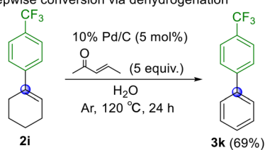
Fig. 5 One-pot biaryl synthesis from 1-arylcylohexanols: construction of benzene rings via Pd/C-catalyzed dehydration and dehydrogenation.
