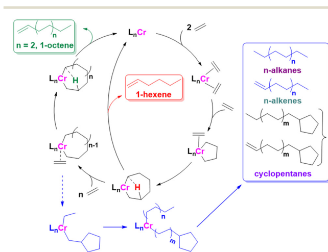
Scheme 1 Ethylene oligomerization via the metallocyclic mechanism. 3,10,11
