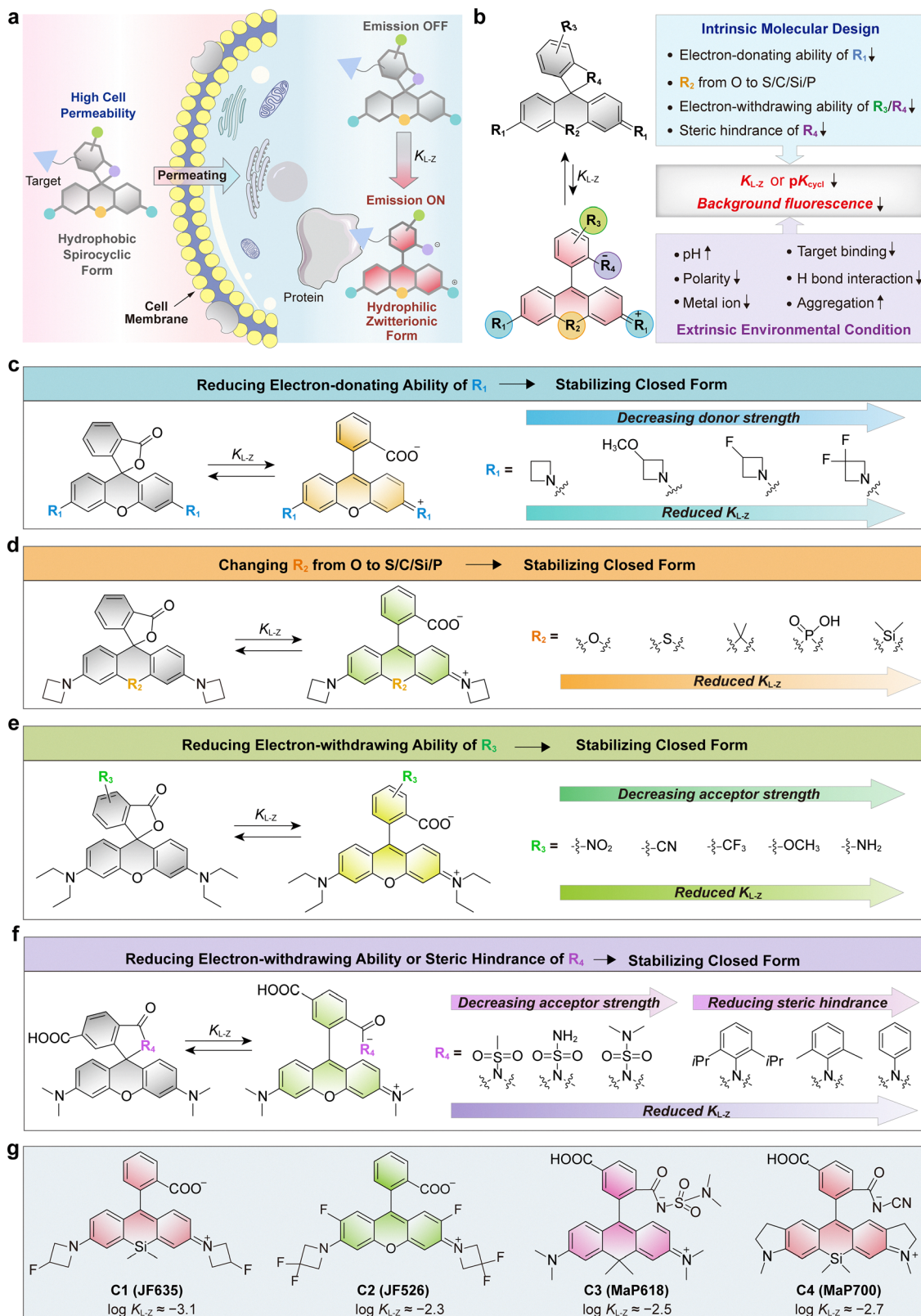
Fig. 18 (a) Schematic illustration of protein labeling-induced ring opening of rhodamines, converting the closed, non-emissive spiroactone (or spirolactam) form into the open, zwitterionic or cationic emissive form. (b) Intrinsic molecular design strategies and extrinsic factors that favor the spirocyclization equilibrium toward the closed form. (c)–(f) Various molecular design strategies to stabilize the closed form of rhodamines. (g) Chemical structures of representative rhodamines and their \log K_{L-Z} values.
