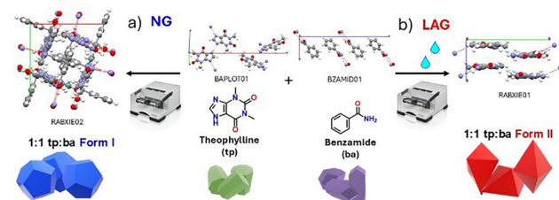
Fig. 7 Selected cocrystal model reaction. 1 : 1 Theophylline : benzamide cocrystal obtained from equimolar mixtures of theophylline anhydrous (tp) and benzamide (ba). (a) Forming 1 : 1 tp : ba Form I (in blue) under NG conditions; (b) 1 : 1 tp : ba Form II (in red) under LAG conditions. 10
