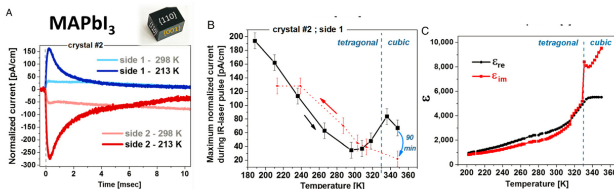
Fig. 9 Relative permittivity and pyroelectric response measurements. (a) Pyroelectric response, J_{\text{pyro}} , in the direction of (001), (b) the pyroelectric character of MAPbI 3 derived from the peak-current value reliance on temperature. Reproduced with permission. 321 Copyright 2011, Macmillan Publishers Limited.
