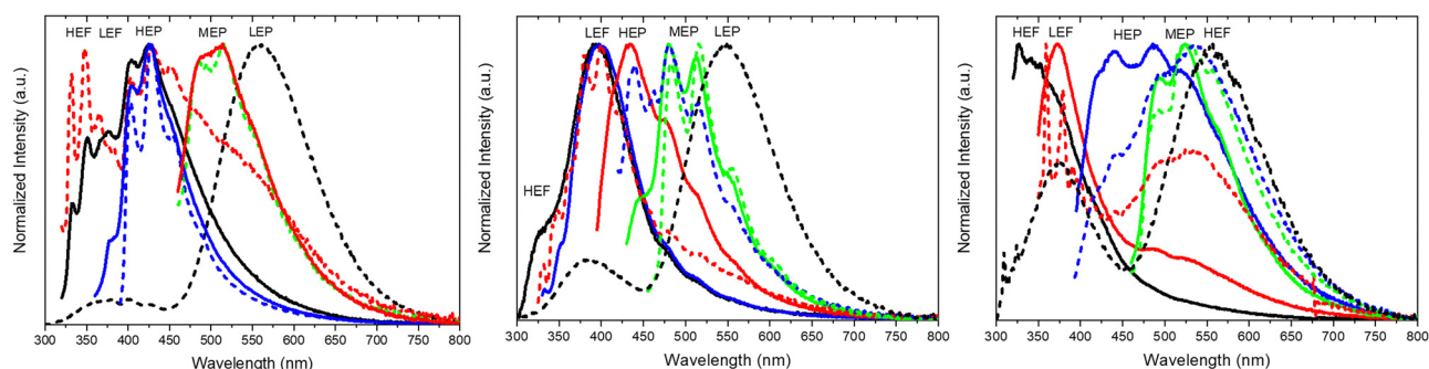
Fig. 7 Normalized PL emission spectra of 1–3Cl crystals at 298 K (full lines) and 77 K (dashed lines). Left 1Cl , 298 K: \lambda_{\text{exc}} = 300 nm (black), \lambda_{\text{exc}} = 340 nm (blue) and \lambda_{\text{exc}} = 440 nm (red). 77 K: \lambda_{\text{exc}} = 280 nm (black), \lambda_{\text{exc}} = 300 nm (red), \lambda_{\text{exc}} = 370 nm (blue) and \lambda_{\text{exc}} = 440 nm (green). Middle 2Cl , 298 K: \lambda_{\text{exc}} = 280 nm (black), \lambda_{\text{exc}} = 308 nm (blue), \lambda_{\text{exc}} = 375 nm (red) and \lambda_{\text{exc}} = 413 nm (green). 77 K: \lambda_{\text{exc}} = 280 nm (black), \lambda_{\text{exc}} = 308 nm (red), \lambda_{\text{exc}} = 400 nm (blue) and \lambda_{\text{exc}} = 434 nm (green). Right 3Cl , 298 K: \lambda_{\text{exc}} = 300 nm (black), \lambda_{\text{exc}} = 330 nm (red), \lambda_{\text{exc}} = 374 nm (blue) and \lambda_{\text{exc}} = 440 nm (green). 77 K: \lambda_{\text{exc}} = 280 nm (black), \lambda_{\text{exc}} = 330 nm (red), \lambda_{\text{exc}} = 373 nm (blue) and \lambda_{\text{exc}} = 440 nm (green).
