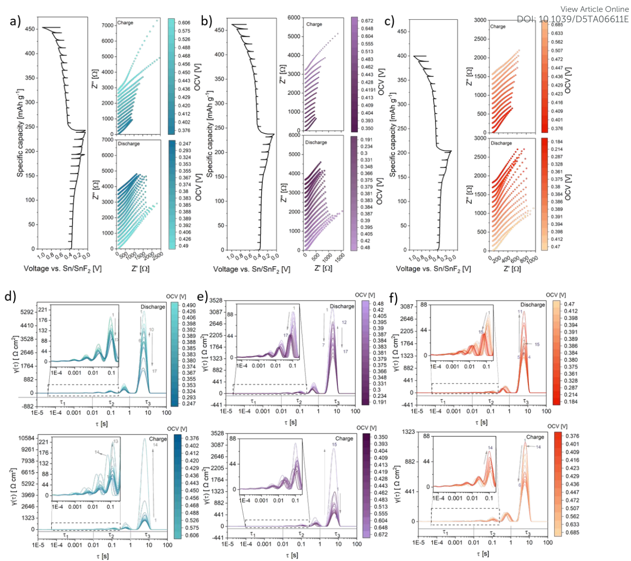
Figure 4 In-situ EIS-DRT analysis of the \text{BiF}_3|\text{BaSnF}_4|\text{Sn} cells under stacking pressures. a) 22 MPa (left) Voltage profile with selected SOCs and (right) corresponding Nyquist plots during discharge and charge; b) 180 MPa (left) Voltage profile with selected SOCs and (right) corresponding Nyquist plots during discharge and charge; c) 430 MPa (left) Voltage profile with selected SOCs and (right) corresponding Nyquist plots during discharge and charge; d-f) Corresponding DRT patterns of the cells in a-c) with specific time constant regimes indicated (SE resistance is determined by the intercept of Nyquist plots at real impedance axis and is not included in DRT analysis due to the absence of a semicircle.)
