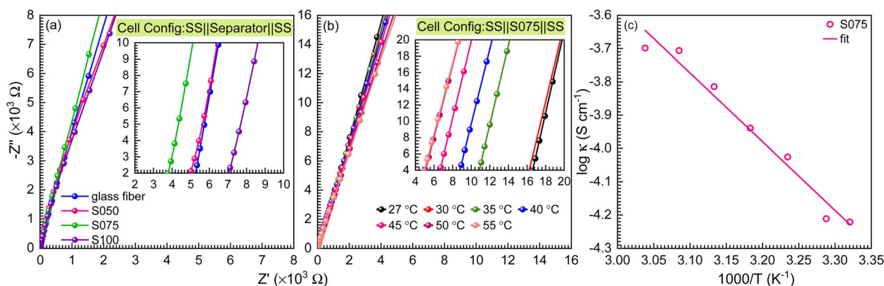
Fig. 4 (a) The Nyquist plot for all the separators at room temperature; (b) the Nyquist plot for the control, S075 membrane at the various temperatures (27 °C, 30 °C, 35 °C, 40 °C, 45 °C, 50 °C, 55 °C), using a blocking electrode system (SS||separator||SS); (c) the ionic conductivity values for the S075 separator at the different temperatures.
