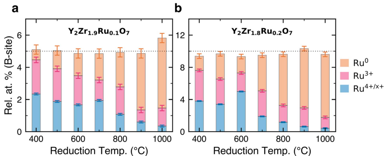
Fig. 5 Relative atomic percentages of the different components of the Ru 3d core level region of Y_2Zr_{1.9}Ru_{0.1}O_7 (a) and Y_2Zr_{1.8}Ru_{0.2}O_7 (b) as a function of reduction temperature. The horizontal dotted lines at 5 at% (a) and 10 at% (b) represent the nominal doping concentration. Error bars were calculated by taking the average of the standard error calculated for three repeat measurements performed on Y_2Zr_{1.8}Ru_{0.2}O_7 samples reduced at 600, 700, 800 and 900 °C.
