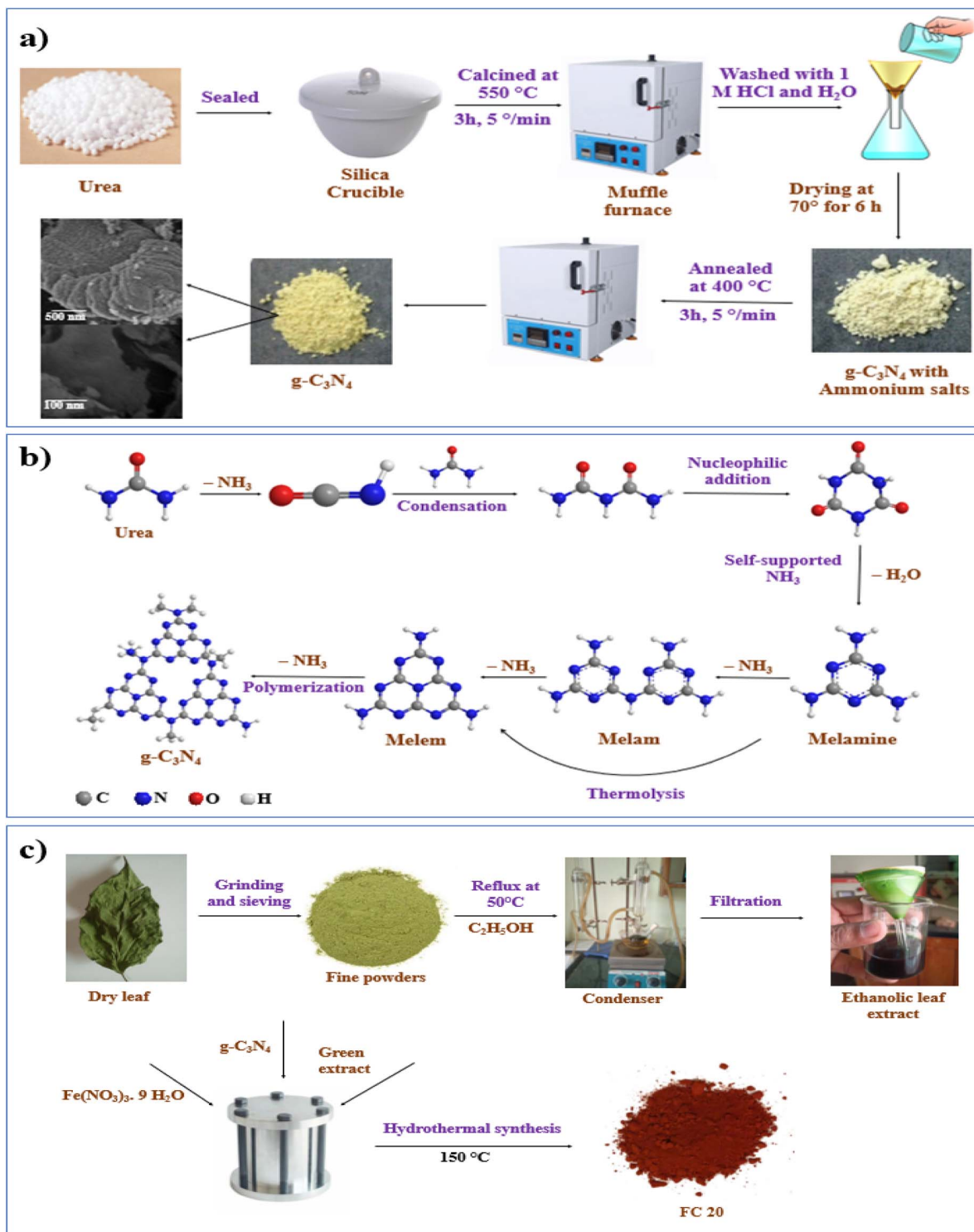
Scheme 1 Graphical representation of catalyst fabrication. (a) Preparation of g-C 3 N 4 ; (b) mechanism of g-C 3 N 4 formation; (c) preparation of α-Fe 2 O 3 /g-C 3 N 4 heterojunction.
