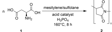
Scheme 1 Thermal polycondensation of aspartic acid 1 to polysuccinimide (PSI) 2.
