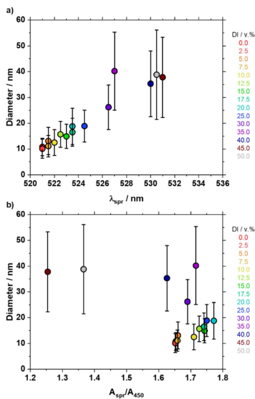
Fig. 2 Diameter as a function of (a) \lambda_{\text{spr}} and (b) A_{\text{spr}}/A_{450} for the Au NPs prepared with various amount of DI water, as indicated. In all cases 0.5 mM \text{HAuCl}_4 and 2 mM NaOH were used for a total of 20 v% ethanol and 80 v% water (DI + mQ).
