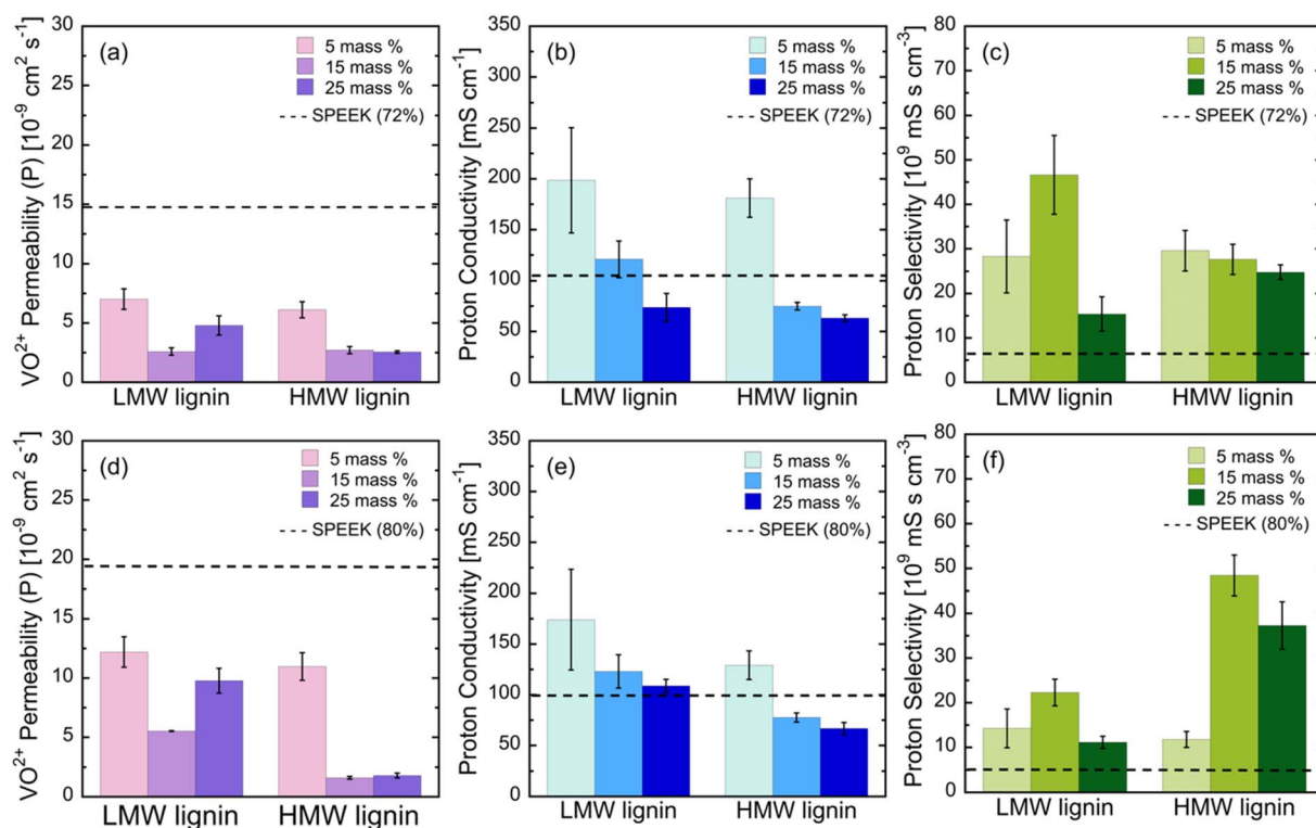
Fig. 2 (a) Vanadyl ion (VO 2+ ) permeability, (b) proton conductivity, and (c) proton selectivity for SPEEK(72%)–lignin nanocomposite membranes. (d) VO 2+ permeability, (e) proton conductivity, and (f) proton selectivity for SPEEK(80%)–lignin nanocomposite membranes. The dashed lines in each figure represent the average value of that property for neat SPEEK membranes. Note, the error bars represent the standard deviation of the average, which was calculated based on measurements on at least three independent membranes.
