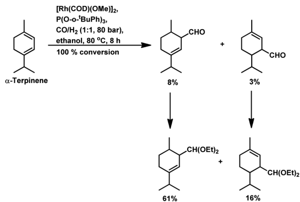
Scheme 13 Hydroformylation/acetalisation of α-terpinene.
