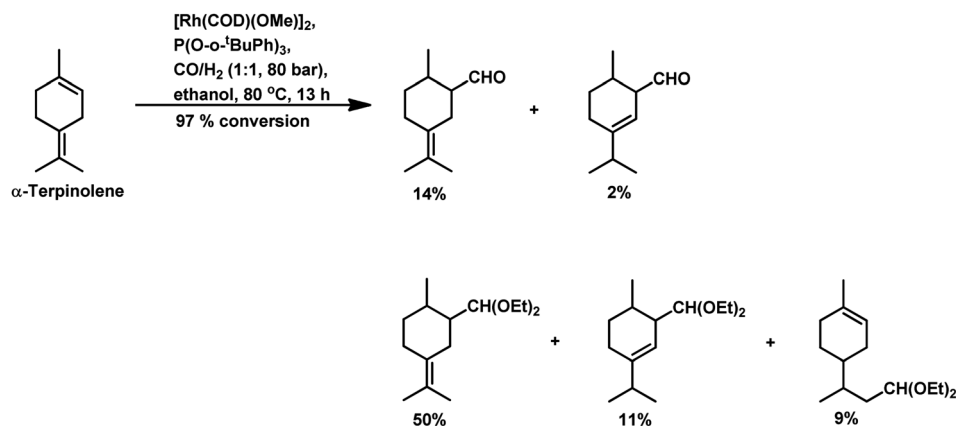
Scheme 15 Hydroformylation/acetalisation of α-terpinolene.
