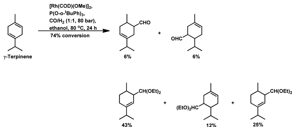
Scheme 14 Hydroformylation/acetalisation of γ-terpinene.
